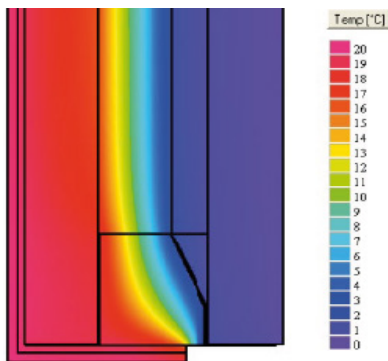
Two-dimensional temperature distribution, highlighting the effectiveness of the thermal break in the lintel.
