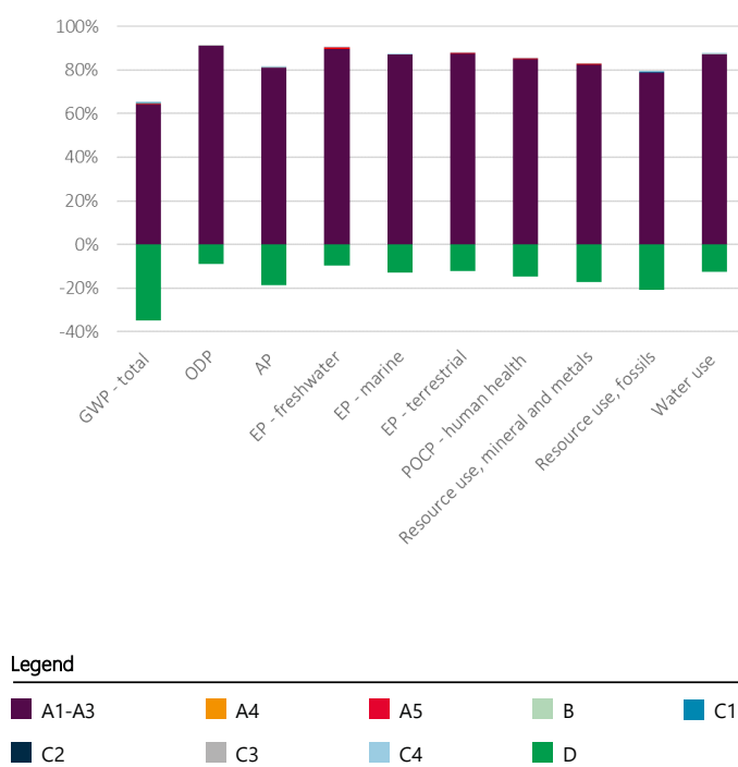
Figure 4 LCA results for Catnic® 390 mm profiles
