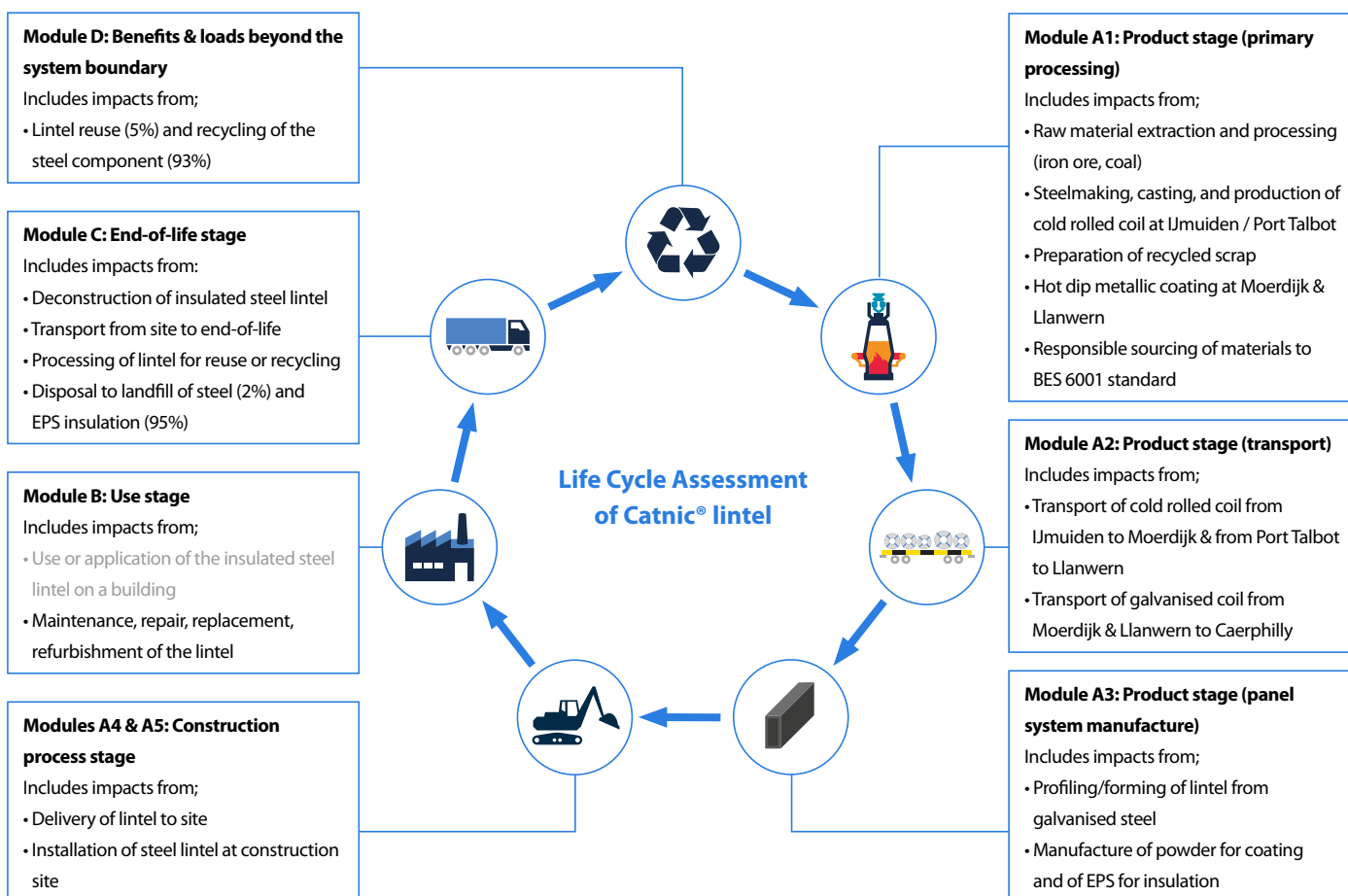
Figure 3 Life Cycle Assessment of Catnic® BSD100 1500 INS lintel
