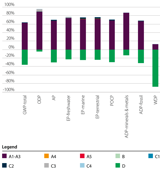
Figure 4 LCA results for Catnic® BSD100 1500 INS lintel
