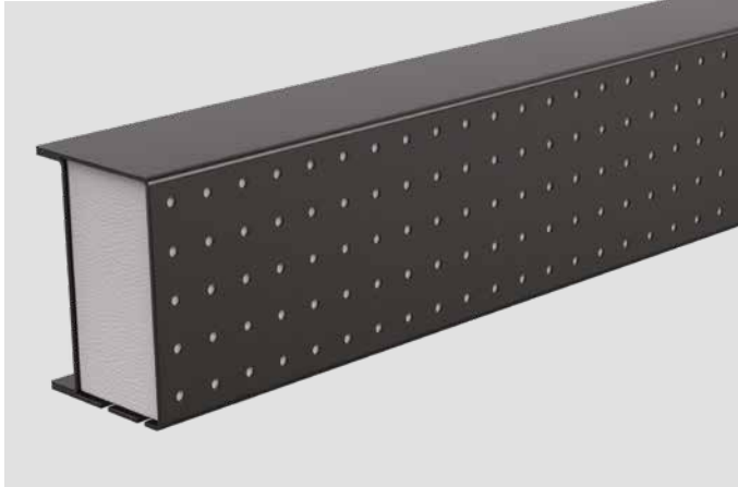
Figure 1 Catnic® BSD100 1500 INS lintel
