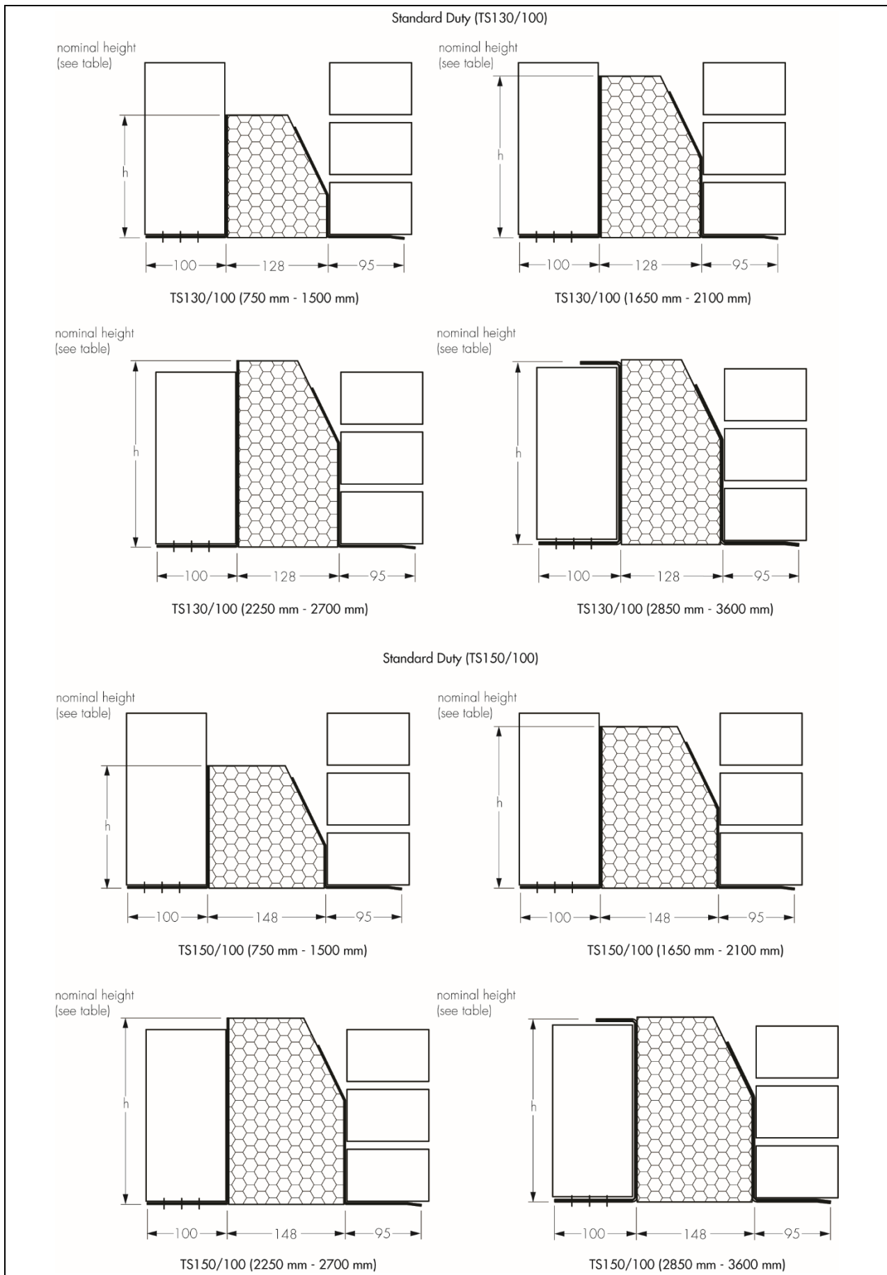
Figure 1 cont'd Typical cross section of TS 90-150 mm thermally broken lintels
