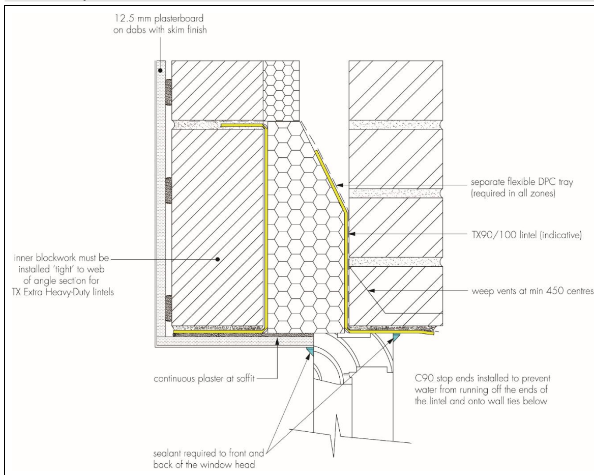
Figure 2 Wall construction incorporating Catnic Thermally Broken Lintels as tested for 30 minutes of resistance to fire
