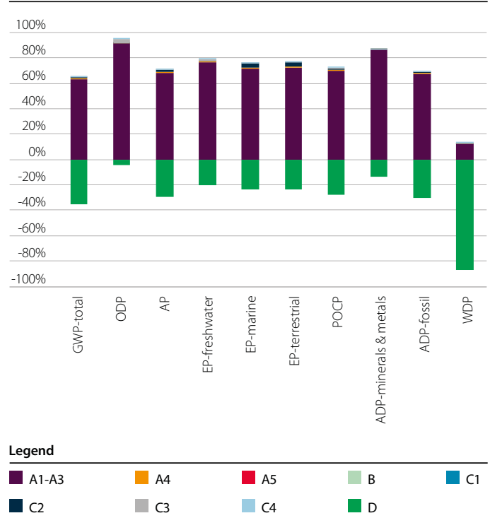
Figure 4 LCA results for Catnic® TS90/1001500 lintel
