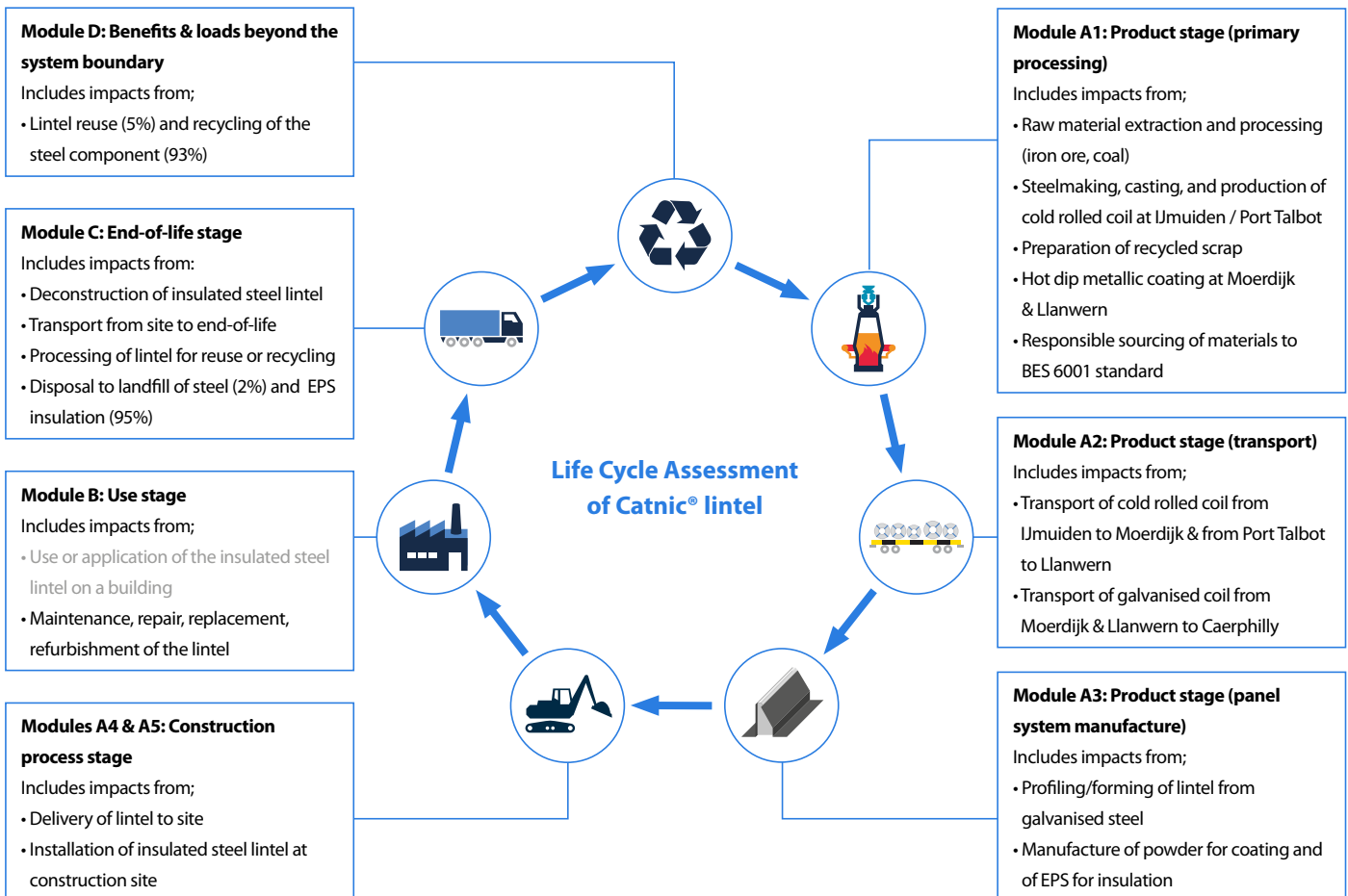
Figure 3 Life Cycle Assessment of Catnic® TS90/1001500 lintel
