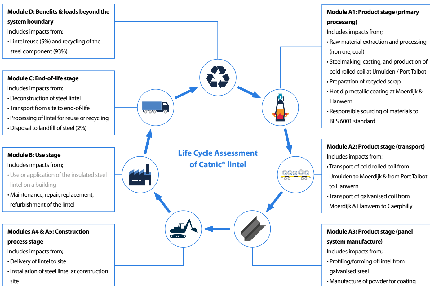
Figure 3 Life Cycle Assessment of Catnic® CTF51500 lintel
