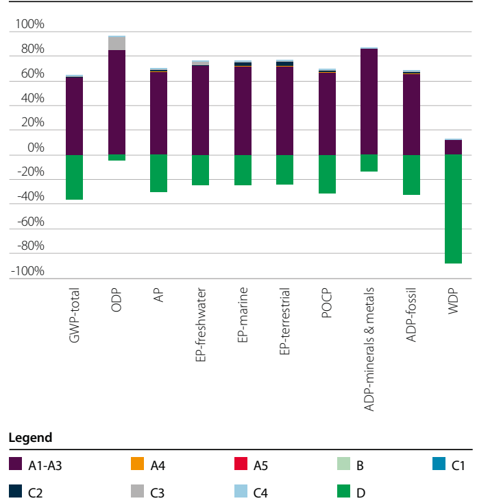
Figure 4 LCA results for Catnic® CTF51500 lintel
