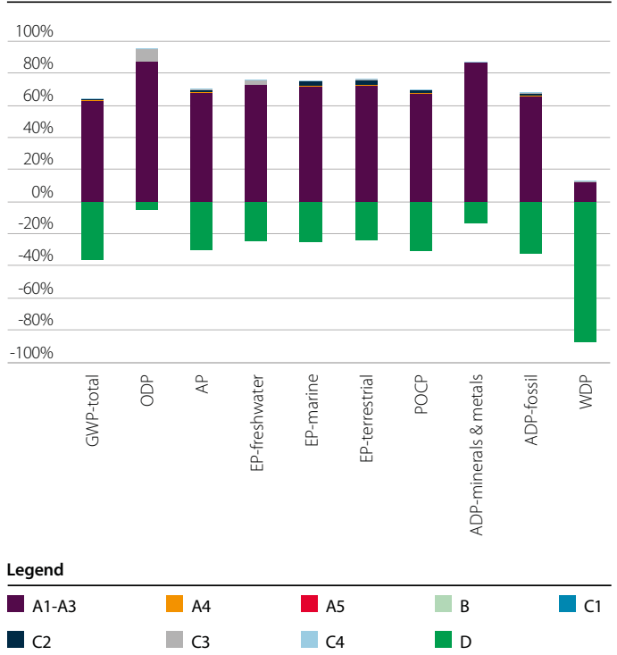
Figure 4 LCA results for Catnic® CH90/1001500 lintel
