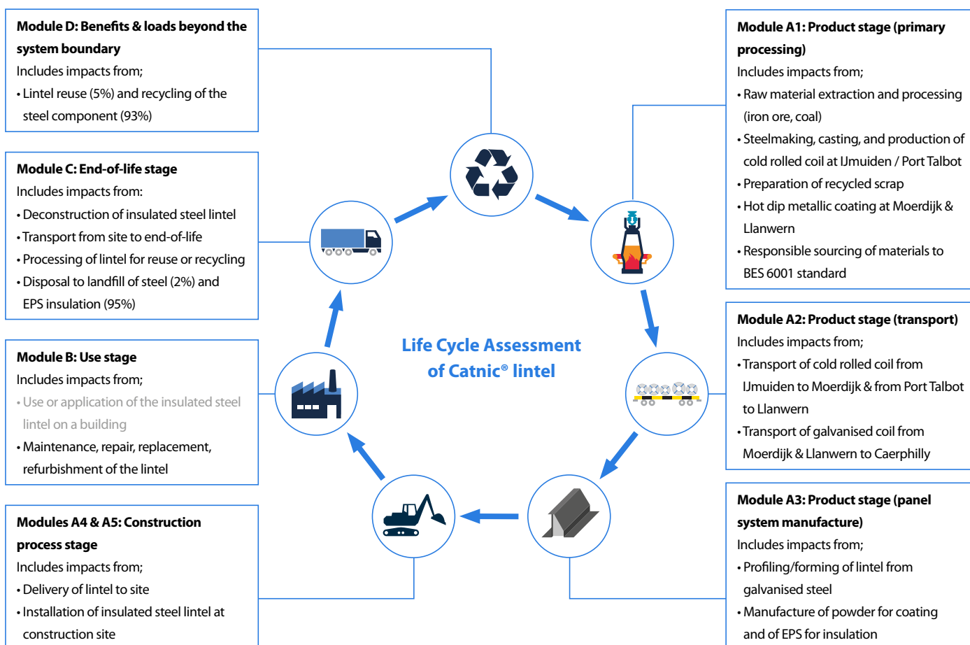
Figure 3 Life Cycle Assessment of Catnic® CH90/1001500 lintel
