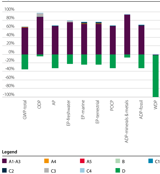
Figure 4 LCA results for Catnic® ANG1500 lintel
